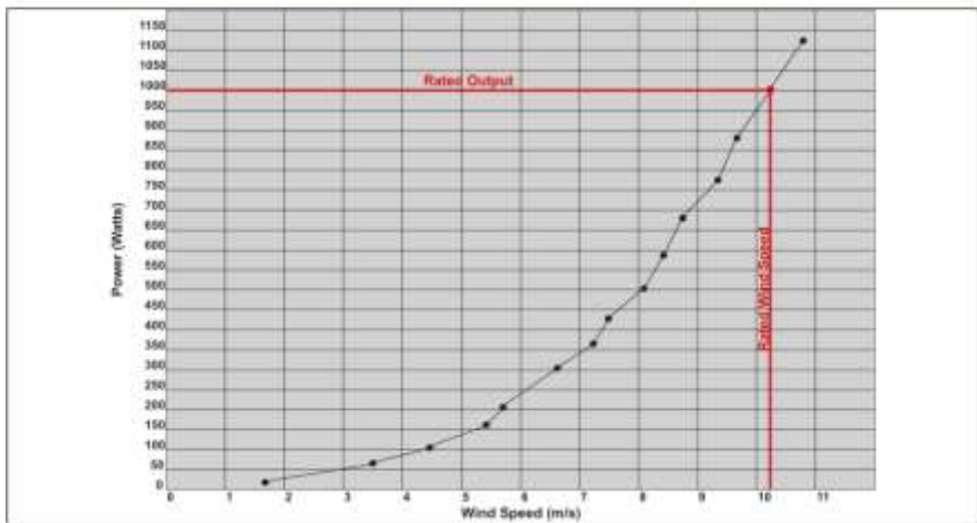
VAWT 1 KW Power Curve
